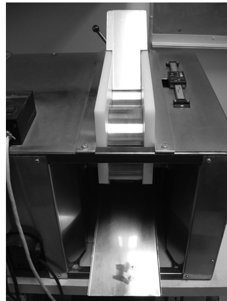
Fig. 1. Laboratory noodle sheeter (75 mm wide rolls).
