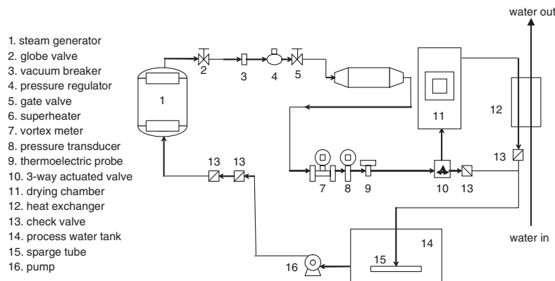
Fig. 2. Schematic of the superheated steam processing system.
