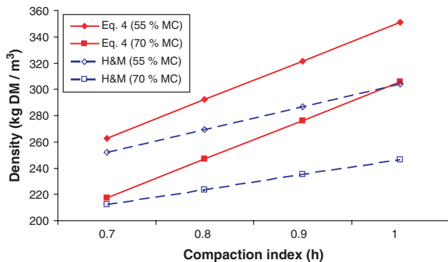
Fig. 3. Predicted average DM density of herbage in a bunker silo as a function of a compaction index (the range 0.7 to 1.0 h is equivalent to a packing tractor mass between 6.2 and 8.9 t for a harvest rate of 8 t DM/h) using the Holmes and Muck (2005) model (H & M) and Eq. 4 at 55 and 70% moisture content (MC).
