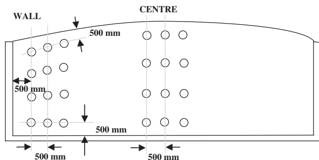
Fig. 1. Core sampling pattern to determine the silage density profile. A total of 48 samples were normally taken at each site and each date from the 24 holes illustrated at two distances from the face: 0 to 180 mm and 180 to 360 mm. Core auger inside diameter was 73 mm (not to scale).
